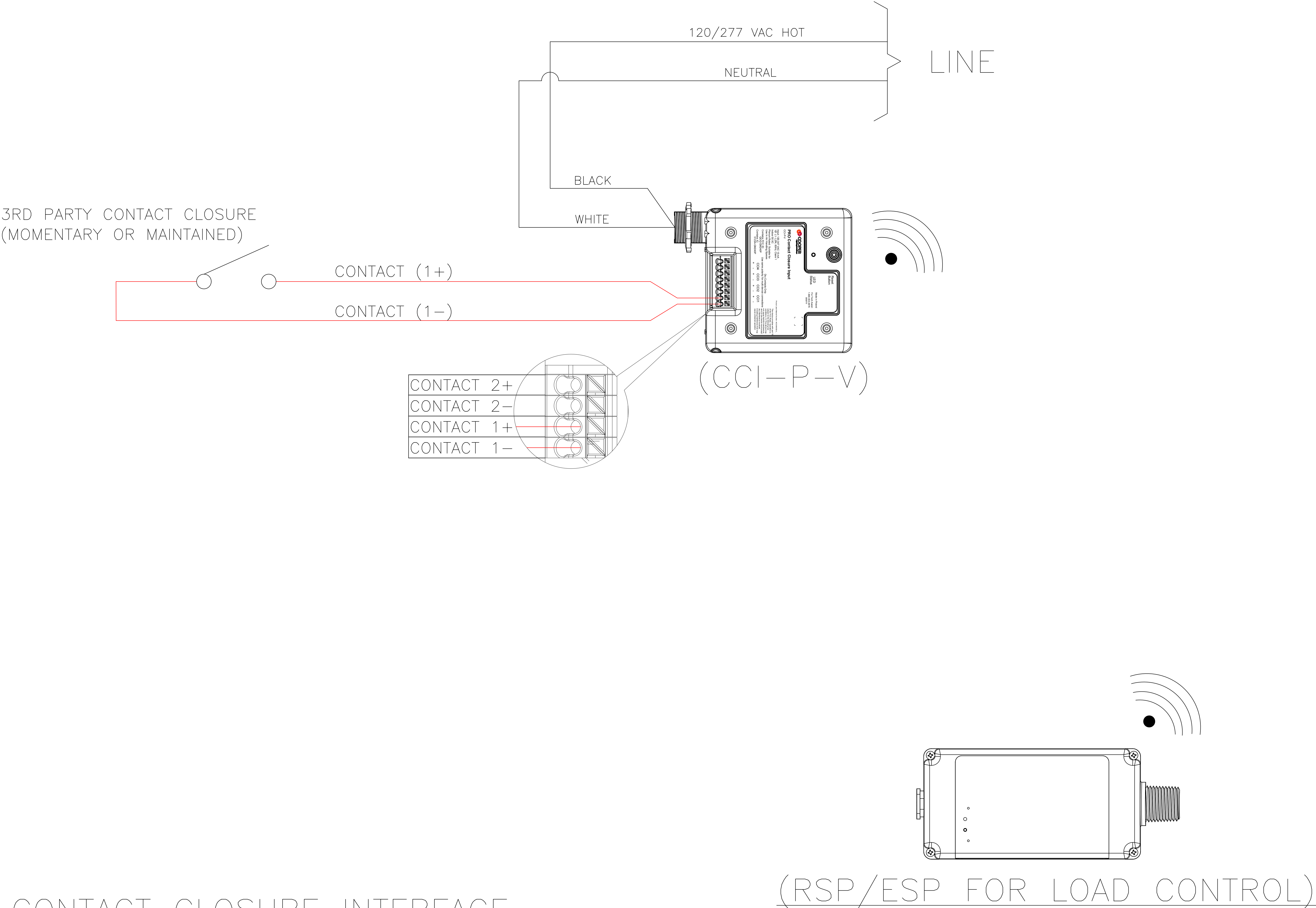
D* 3RD PARTY CONTACT CLOSURE INTERFACE (1)CCI-P-V
