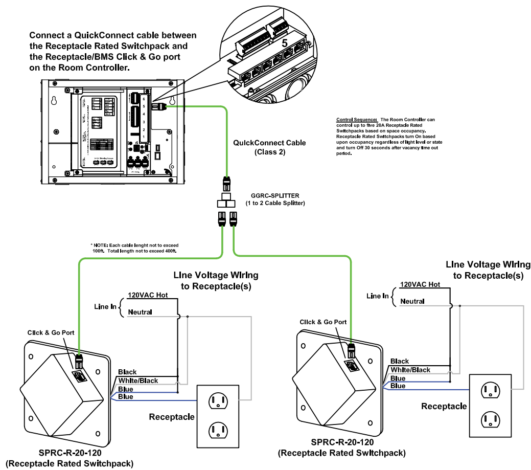
Figure 9: Receptacle wiring
