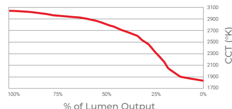
CCT vs current curve for 3000K-1800K
