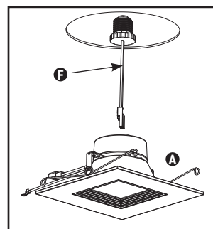
Figure 5 Retrofit
