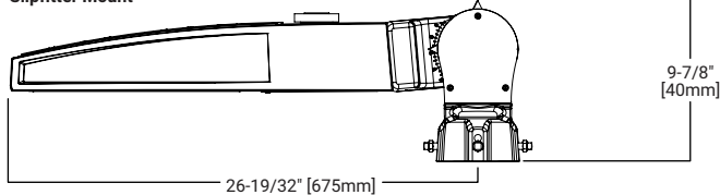
Slipfitter Mount
