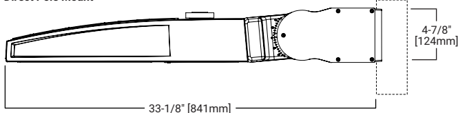
Wall Mount
