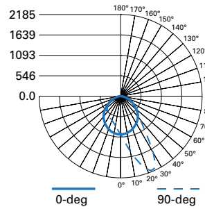
ASYMMETRIC FLUSH LENS
