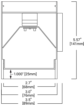
Regressed Housing
