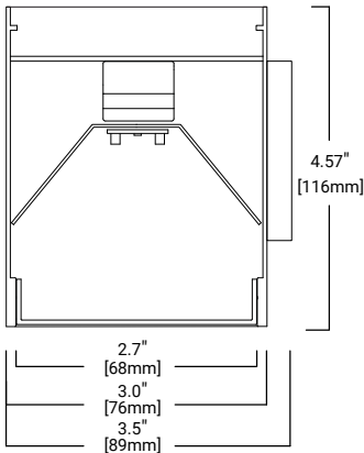
Standard Housing
