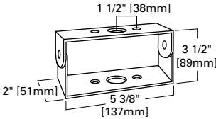
TRUNNION MOUNT
