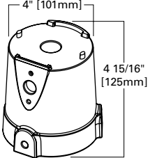
TYS (Slipfitter Adapter)
