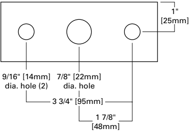
YOKE MOUNT
