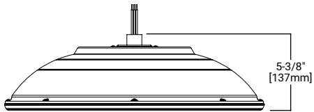
Stem Mount
