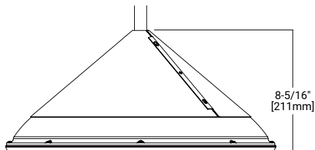
Bird Guard (TT/BG-UP-XX)
