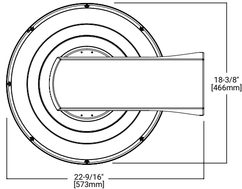
Top View - Wall Mount
