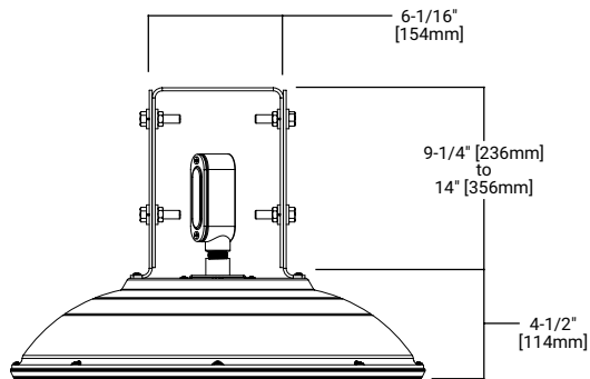
Trunnion Mount
